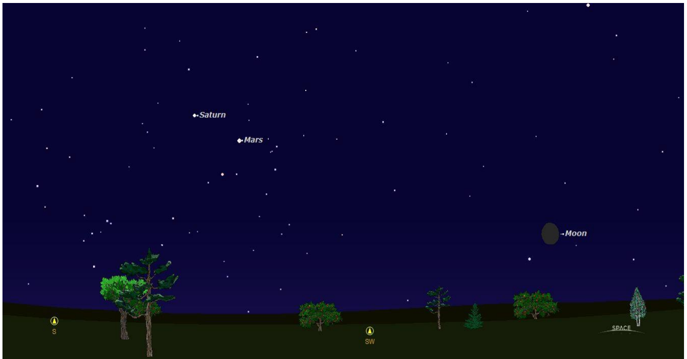
Illustration 2 April 20 th Looking South before sunrise
