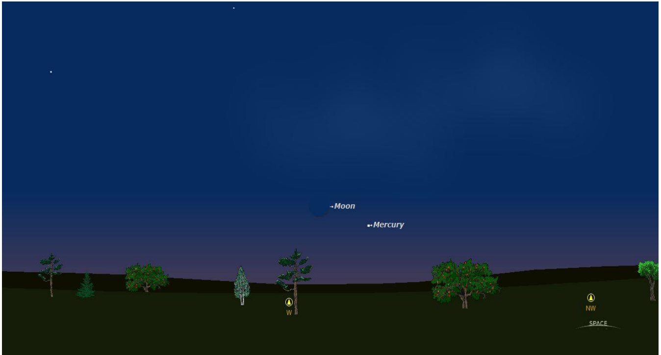
Illustration 1 April 8 th Looking West, Northwest after sunset
