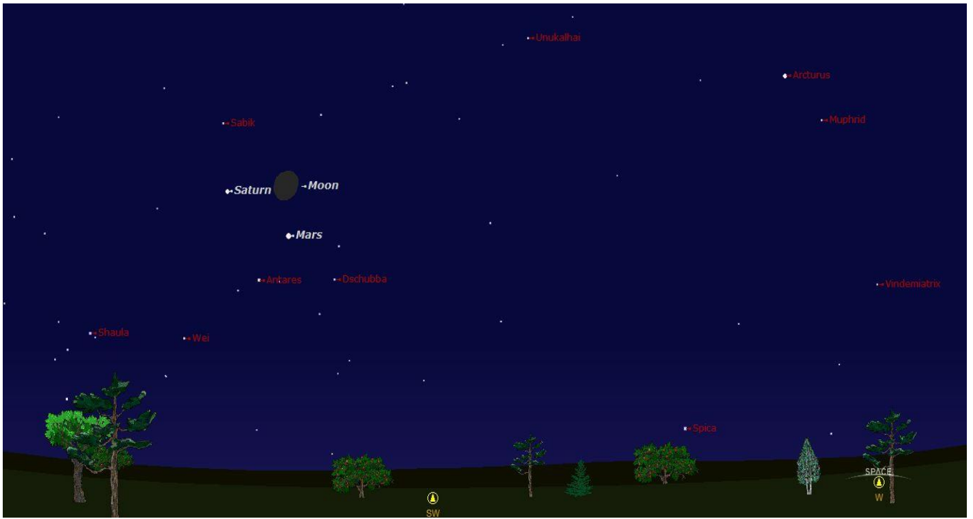
Illustration 3 April 25 th Looking southwest before sunrise
