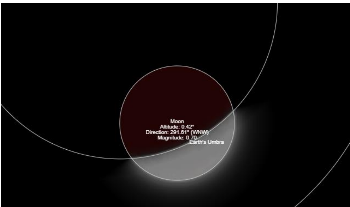
Illustration 2 Maximum Lunar Eclipse 7:35 am
