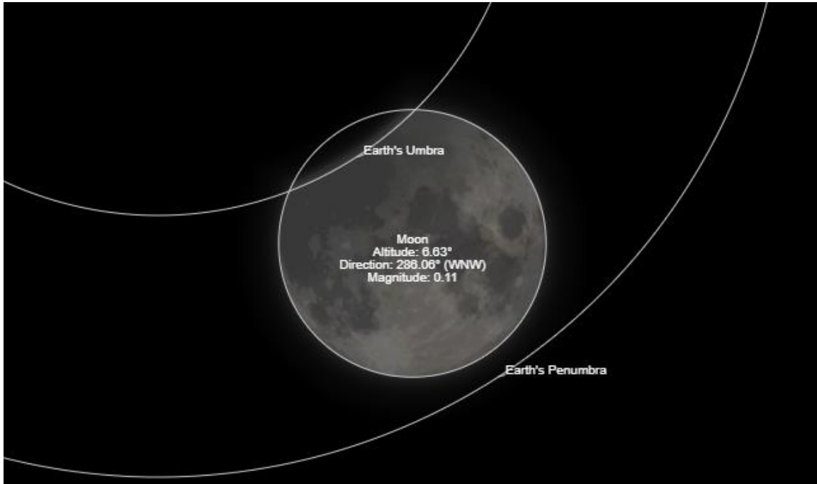
Illustration 1 Partial Lunar Eclipse Begins 6:48 am
